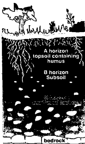
A Horizon and other layers of soil
